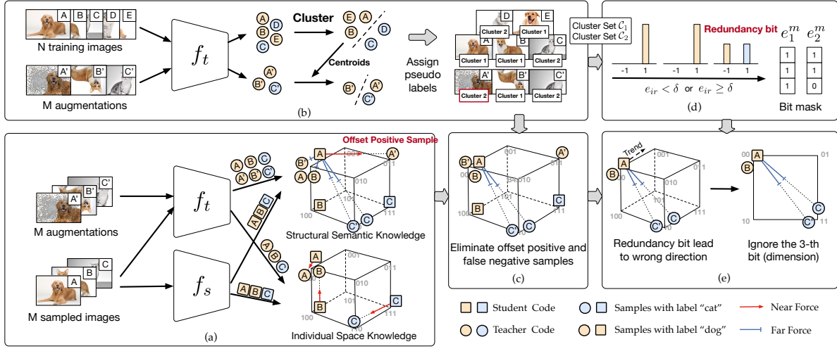
Figure 2: Workflow of BRCD. (a) The contrastive knowledge distillation achieves individual-space and structural-semantic knowledge transfer. (b) Clustering and assigning pseudo labels to images. (c) Cluster-based method eliminates offset positive and false negative samples. (d) The process to get bit masks. (e) Bit mask mechanism prevents incorrect optimization direction.
