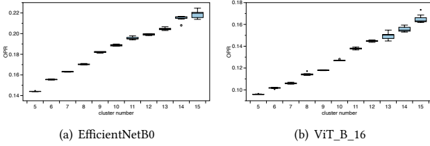
Figure 6: The OPR in the CIFAR-10 dataset when using EfficientNetB0 or ViT_b_16 as the model’s backbone. A higher OPR indicates a greater occurrence of offset positive samples.
