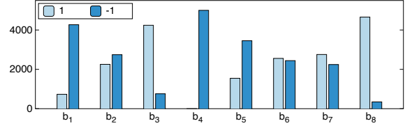
Figure 3: We conduct the analysis using 5000 images with the same class on the CIFAR-10 dataset. It shows the frequency histograms of eight randomly chosen dimensions.
