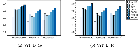
Figure 4: The mAP@1000 results on the CIFAR-10 dataset when using different knowledge methods and backbones.
