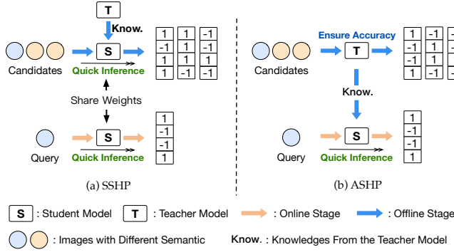
Figure 1: Search paradigms for semantic hashing. (a) represents the Symmetric Semantic Hashing search Paradigm (SSHHP), utilizing a single model for both offline and online stages. (b) depicts the Asymmetric Semantic Hashing search paradigm (ASHHP), employing distinct models for each stage.
