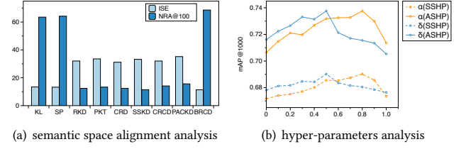
Figure 5: (a) The ISD and NRA@K on CIFAR-10 dataset for semantic space alignment analysis. (b) Hyper-parameters analysis on \alpha and \delta .
